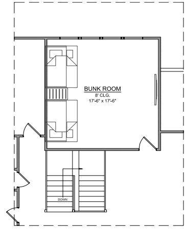
Bunk room Option – Over garage adds – 328 SQ FT
