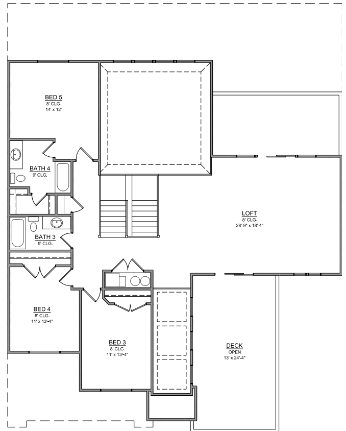
Upper Level 1,446 SQ FT
