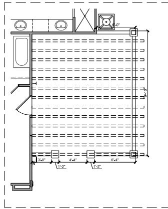
Timber Pergola Option
