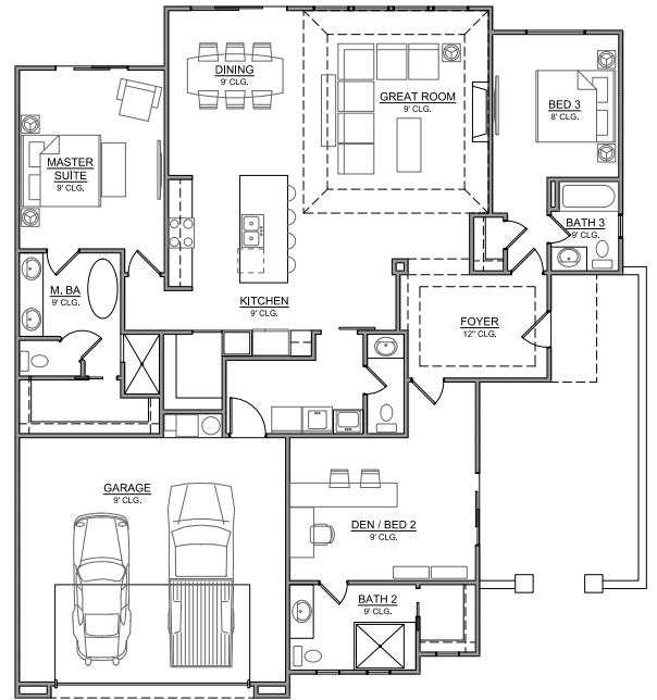
3 Bedroom Option - 1,952 SQ FT
